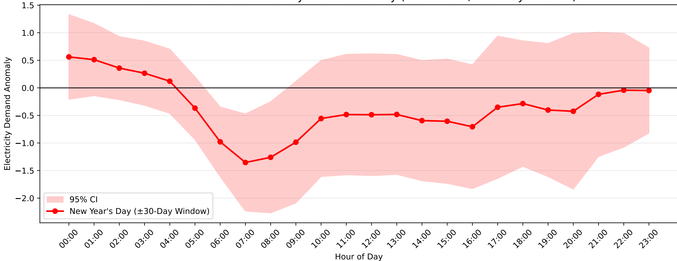
Narrabeen Demand Anomaly: New Year's Day (2004-2017, \pm 30 -Day Window)
